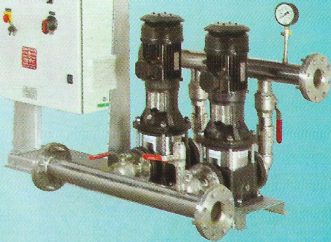
AQUAPACK Hydro-pneumatic Pressure System
